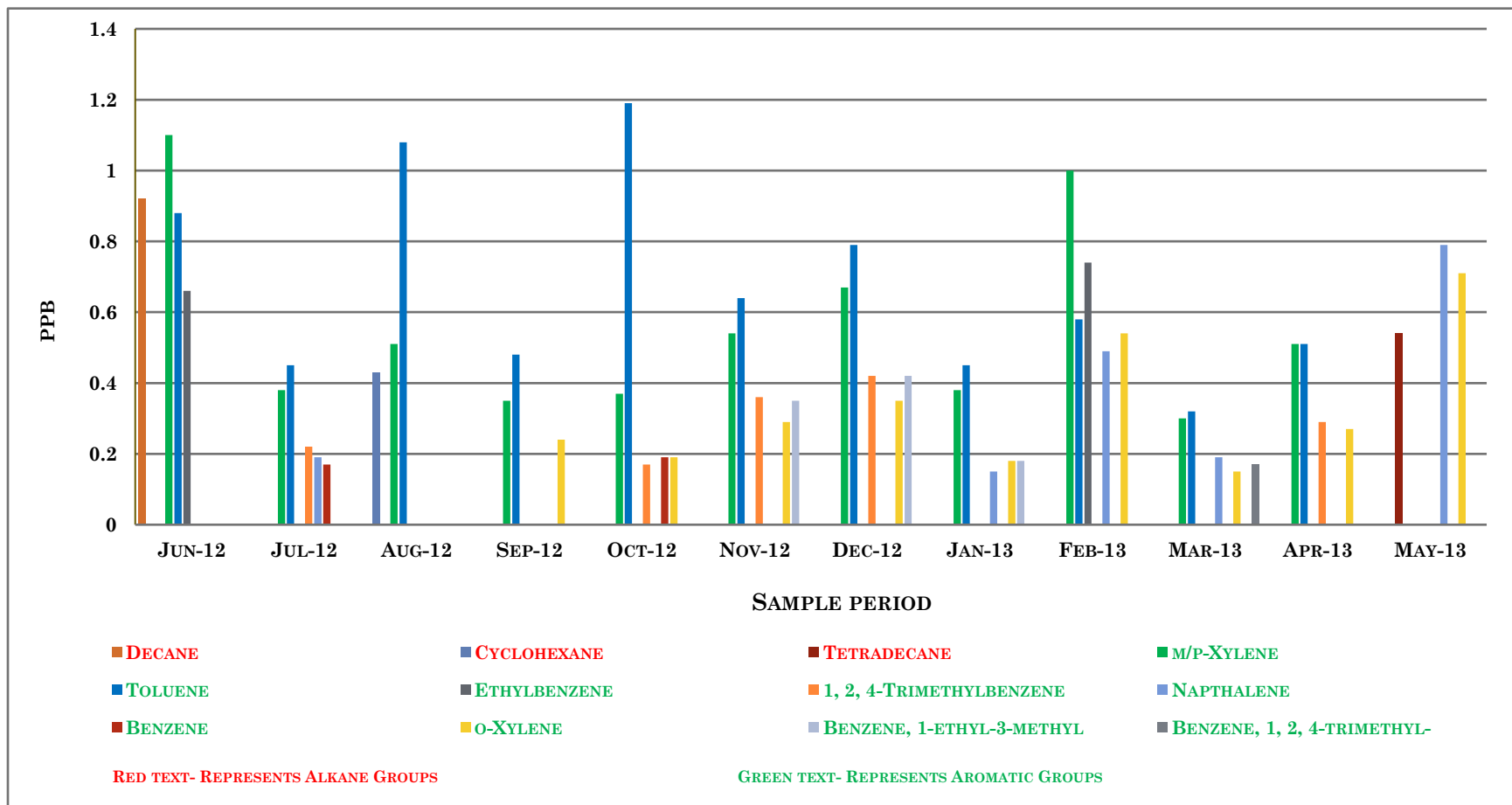
Graph 8: VOC compounds detected at the Pickwick Gap sampling location during the study period June 2012 to May 2013. The compounds shown represent only those compounds covered in the laboratory accredited flexible scope and are not blank corrected.
