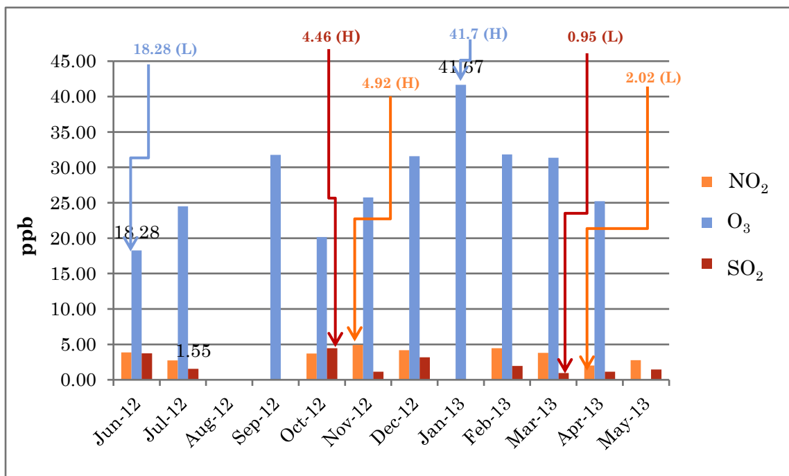
Graph 1: SO 2 , NO 2 and O 3 concentrations for Waterford, St. Michael. (H) represents the highest and (L) represents the lowest value detected.
