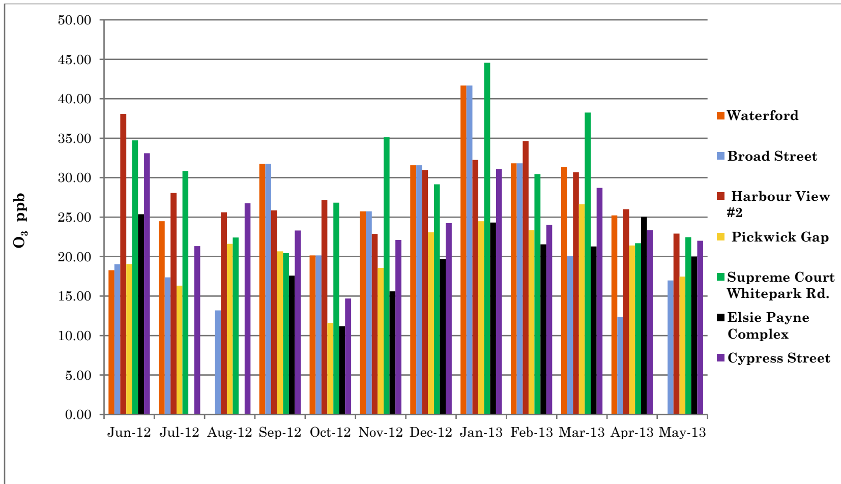
Graph 25: The average O 3 concentration across all sampling locations for the study period
