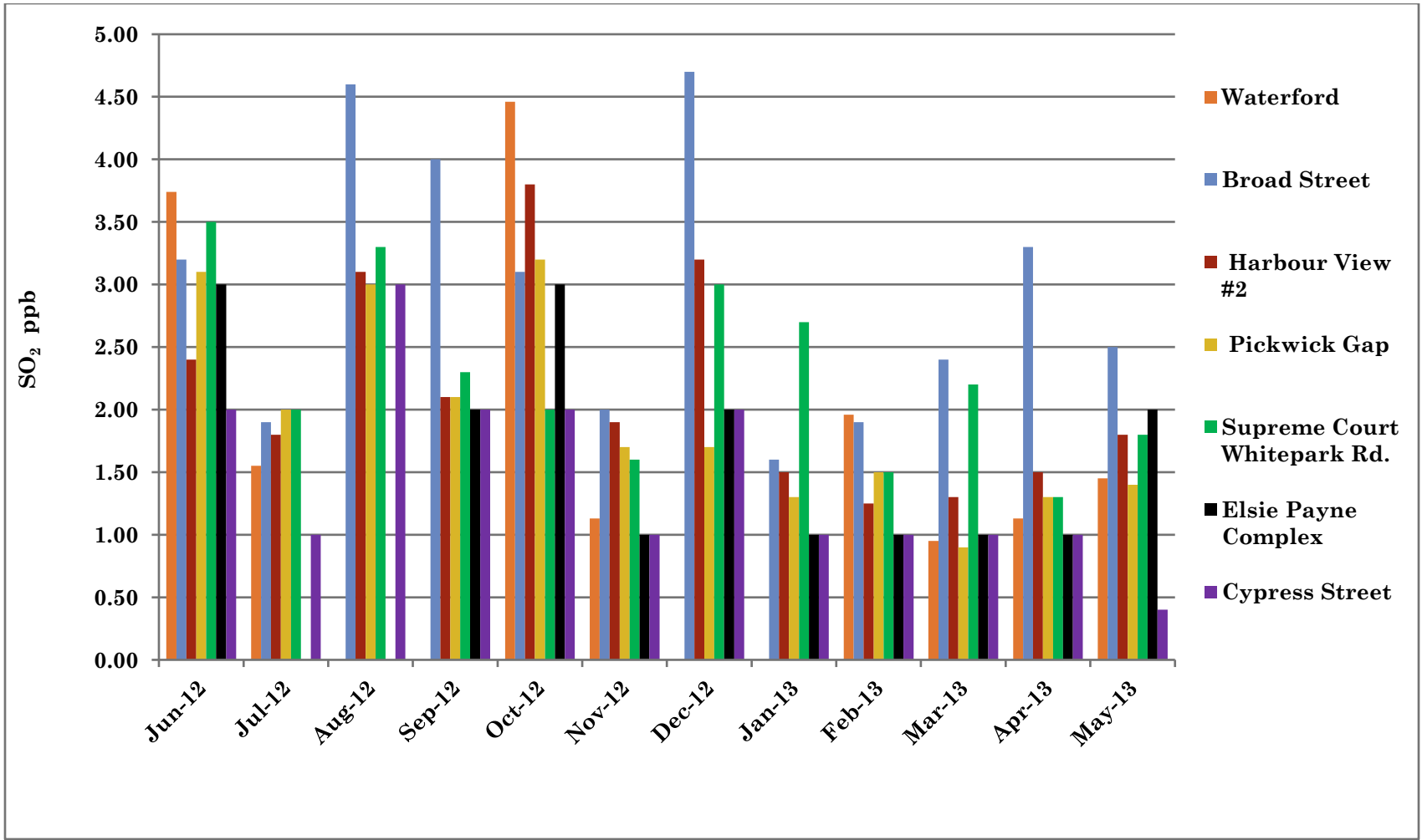
Graph 23: The average SO 2 concentrations across all sampled locations during the study period.
