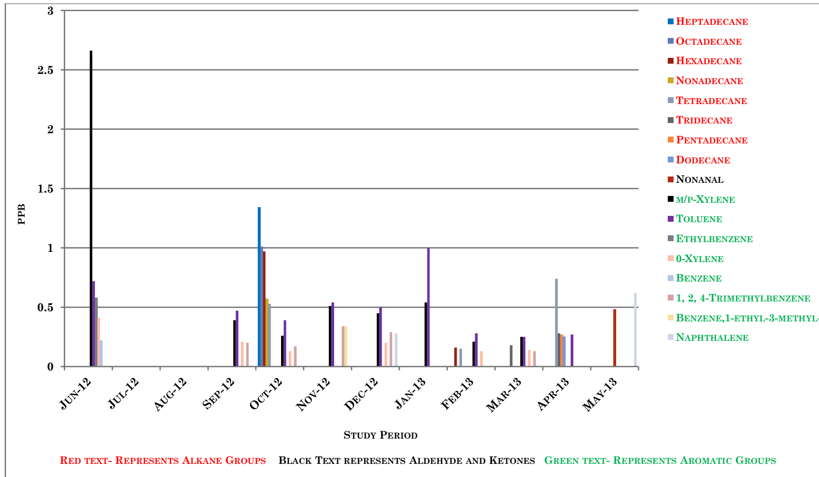
Graph 12: VOC compounds detected at the Supreme Court, Whitepark Rd. sampling location during the study period June 2012 to May 2013. The compounds shown represent only those compounds covered in the laboratory accredited flexible scope and are not blank corrected.
