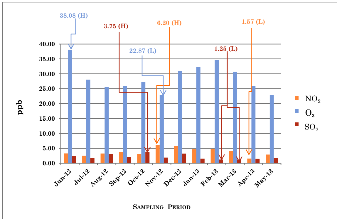
Graph 5: SO 2 , NO 2 and O 3 concentrations at Harbour View # 2. (H) represents the highest and (L) represents the lowest value detected
