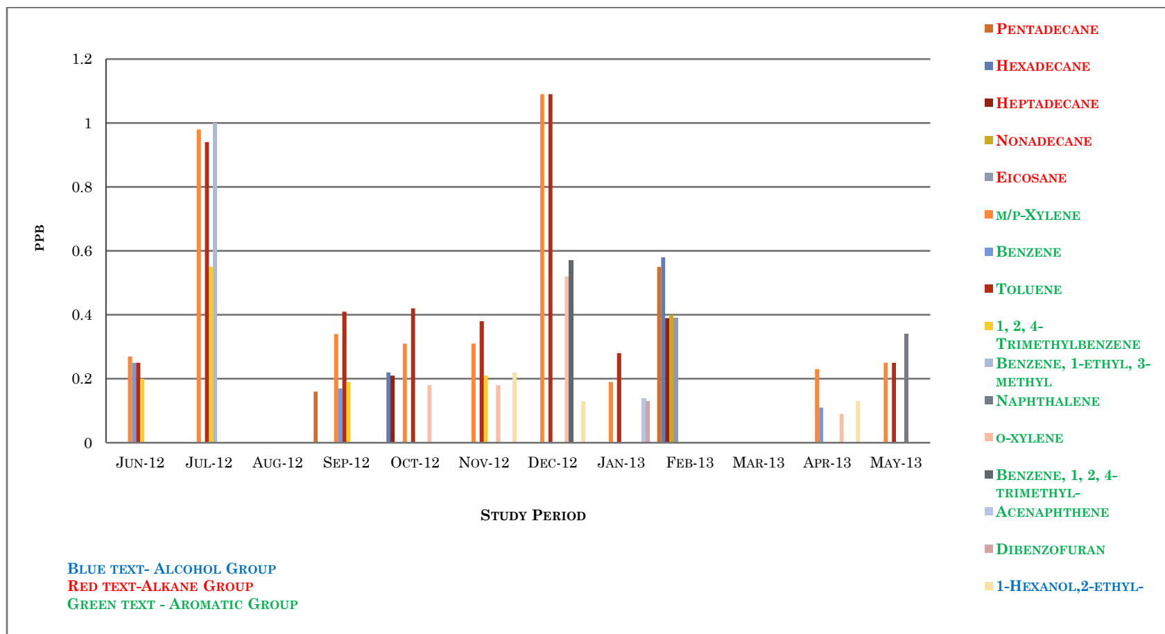
Graph 2: Top Five VOC at the Waterford sample site for the period June 2012 to May 2013. The compounds shown represent only those compounds covered in the laboratory accredited flexible scope and are not blank corrected.
