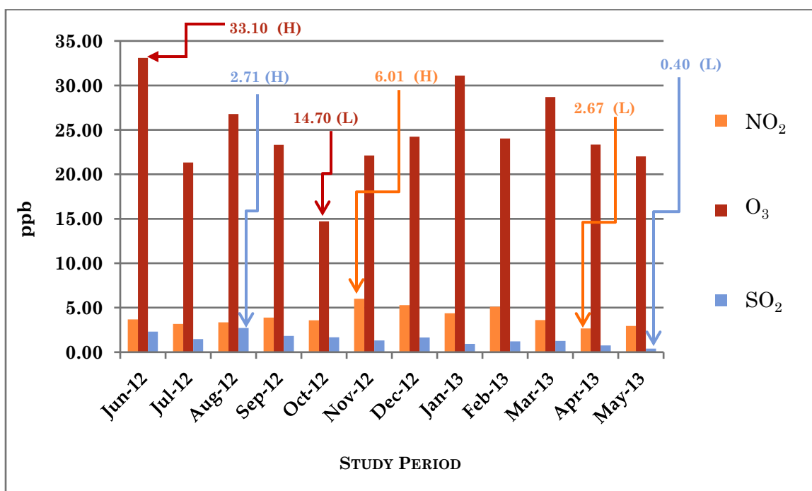
Graph 13: SO 2 , NO 2 , and O 3 concentrations at Cypress Street during the period June 2012 to May 2013. (H) represents the highest and (L) represents lowest values detected.
