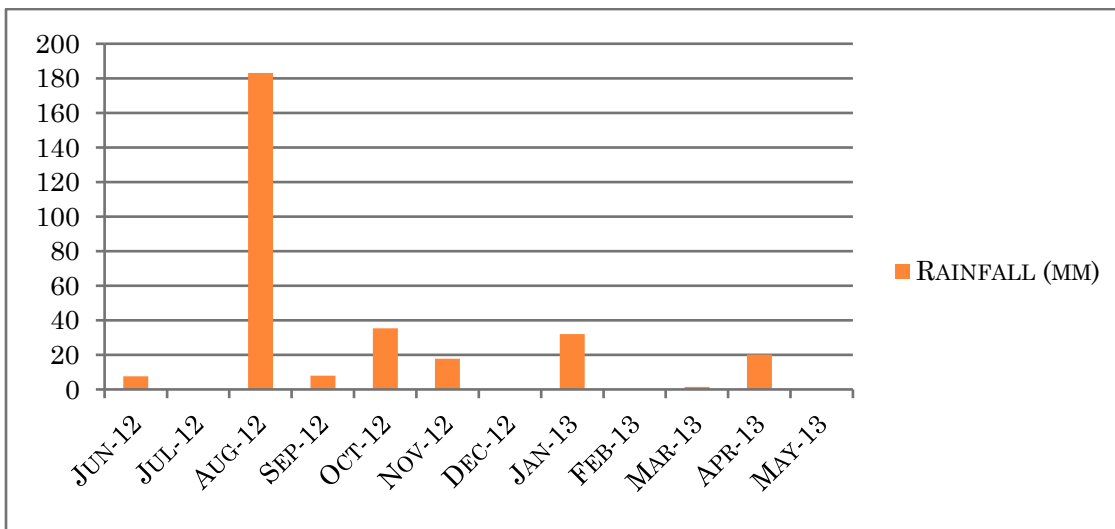
Graph 18: Average monthly rainfall data collected during the period June 2012 to May 2013 as provided by CZMU weather stations.
