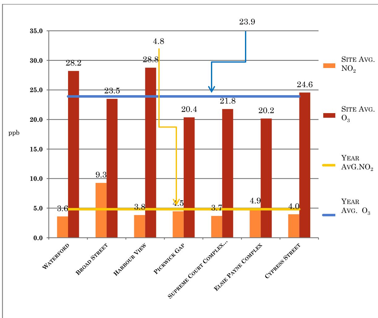
Graph 22: The average NO 2 and O 3 concentrations per location.
