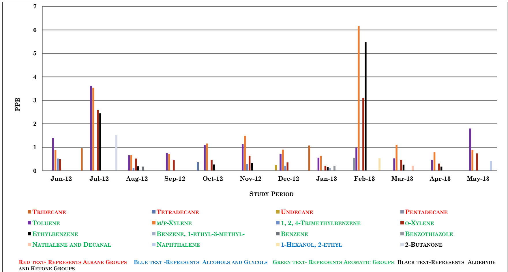
Graph 6: VOC compounds detected at the Harbour View #2 sampling location during the study period June 2012 to May 2013. The compounds shown represent only those compounds covered in the laboratory accredited flexible scope and are not blank corrected.
