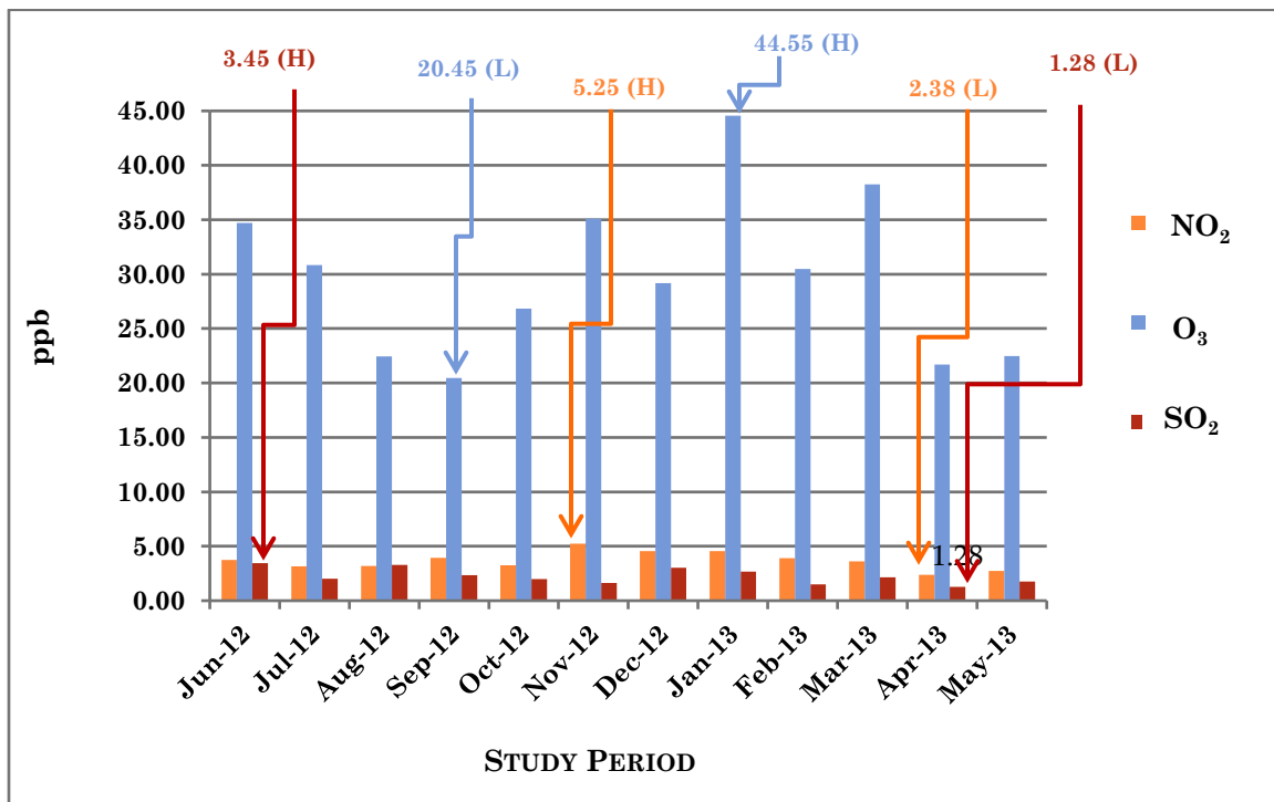
Graph 9: NO 2 and O 3 concentrations at the Supreme Court Complex, Whitepark Rd, St. Michael. (H) represents the highest and (L) represents lowest values detected
