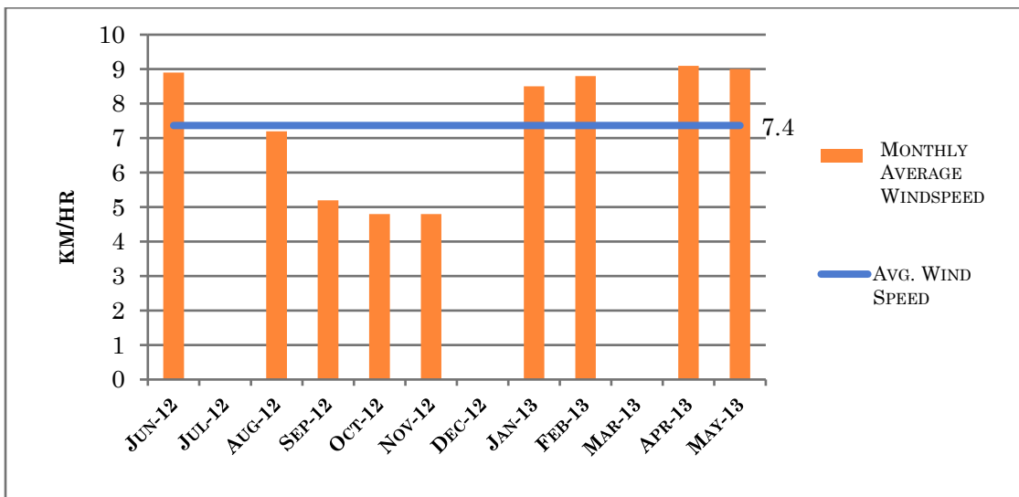
Graph 17: Average wind-speed (km/h) for the period sampled.
