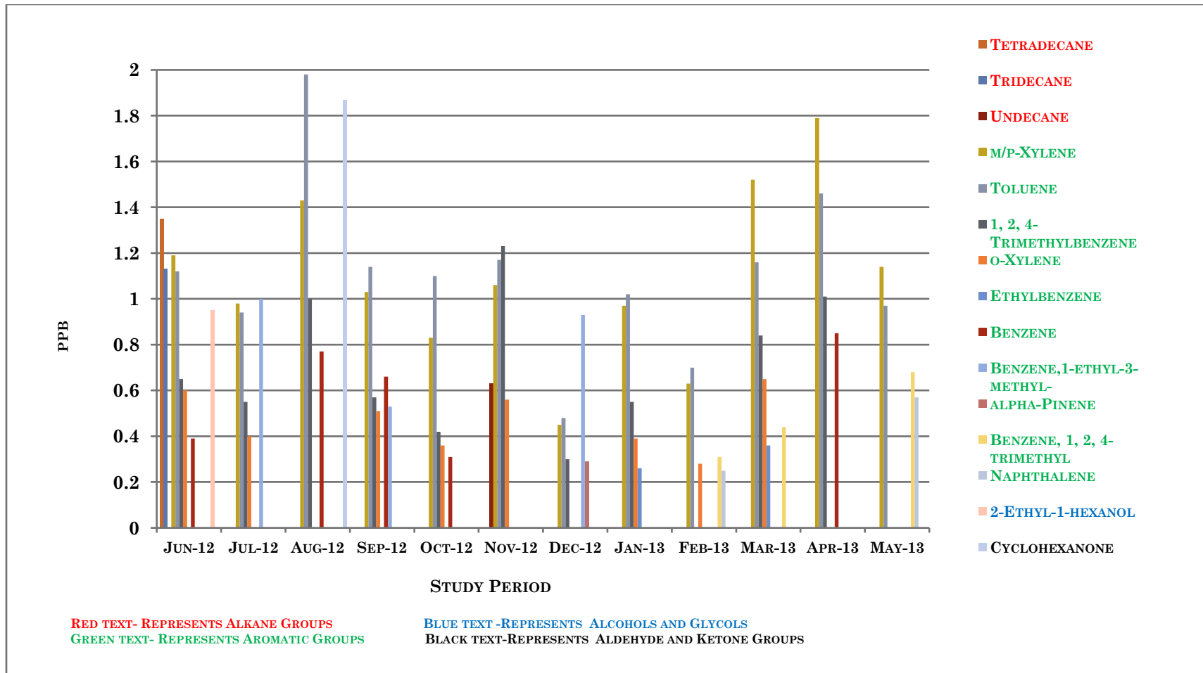
Graph 4: VOC compounds detected at the Broad Street sampling location during the study period June 2012 to May 2013. The compounds shown represent only those compounds covered in the laboratory accredited flexible scope and are not blank corrected.
