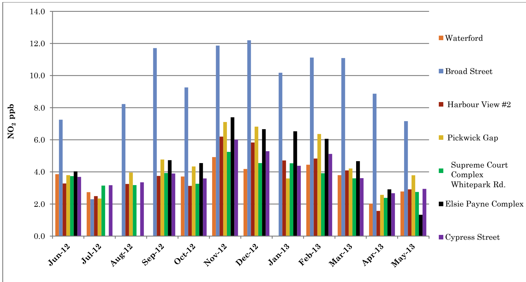
Graph 24: Average NO 2 concentrations for the study period for all sample locations.
