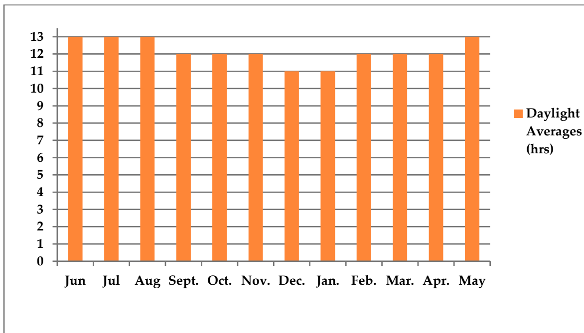
Graph 19: Daylight averages for Barbados
