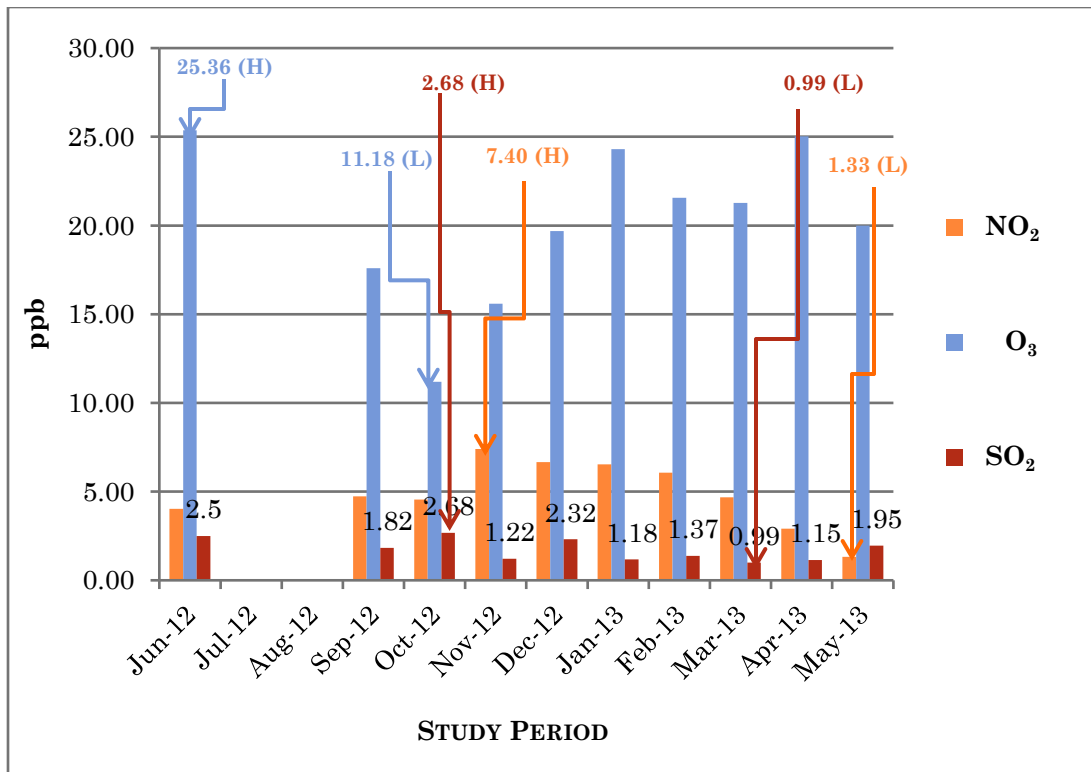
Graph 11: SO 2 , NO 2 and O 3 concentrations for the Queen’s Park/Elsie Payne Complex. (H) represents the highest and (L) represents lowest values detected.
