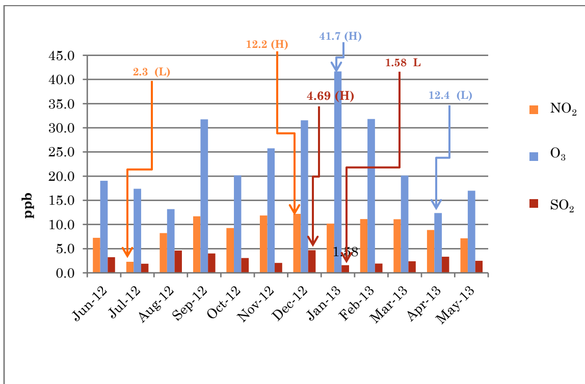
Graph 3 SO 2 , NO 2 and O 3 levels for Broad Street, Bridgetown, (H) represents the highest and (L) represents the lowest value detected
