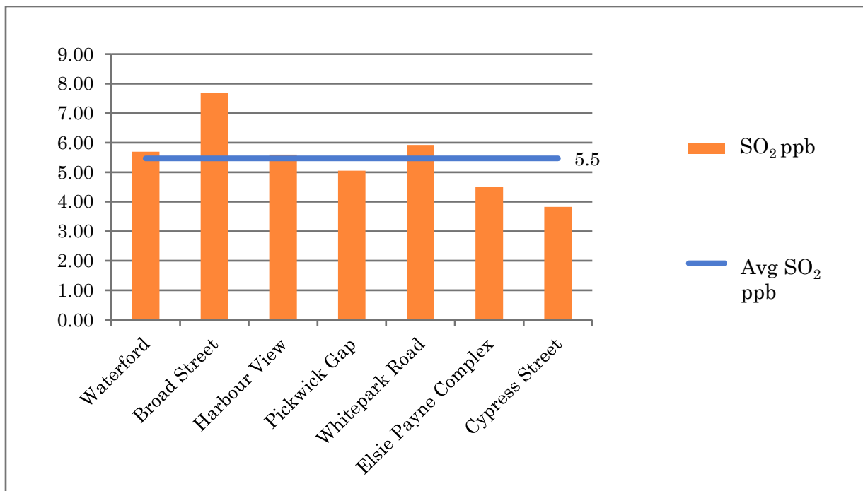
Graph 21: Average SO 2 levels per location in µg/m 3 .
