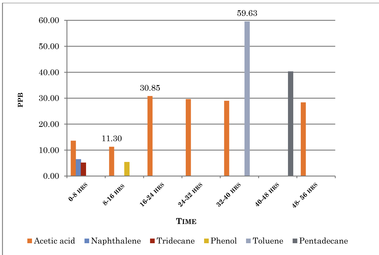
Graph 15: Highlights those compounds detected at Harbour View #2 within the flexible scope and not those compounds which may be a result of the reaction of the Tenax sorbent with Ozone and are not blank corrected.
