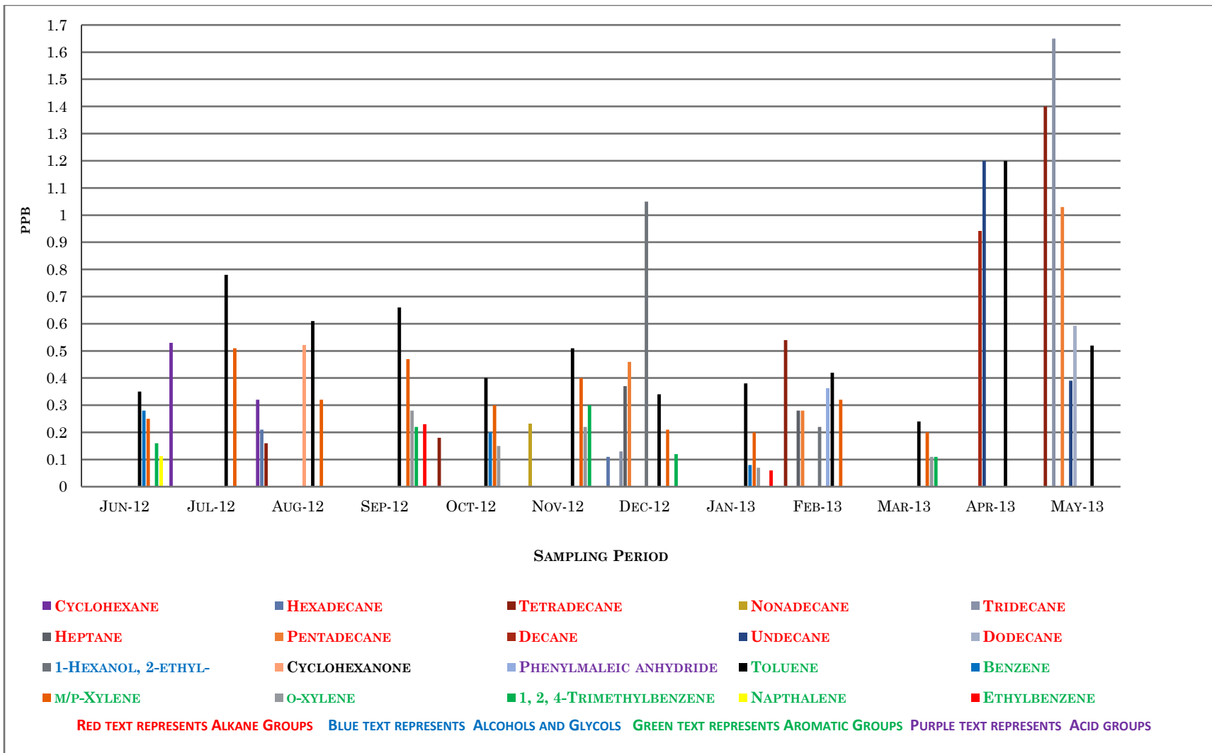
Graph 10: VOC compounds detected at the Supreme Court, Whitepark Rd. sampling location during the study period June 2012 to May 2013. The compounds shown represent only those compounds covered in the laboratory accredited flexible scope and are not blank corrected.
