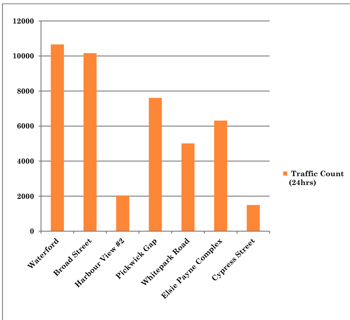
Graph 20: Traffic volume per 24 hours. Peak traffic was observed at both Waterford main road and along Broad Street
