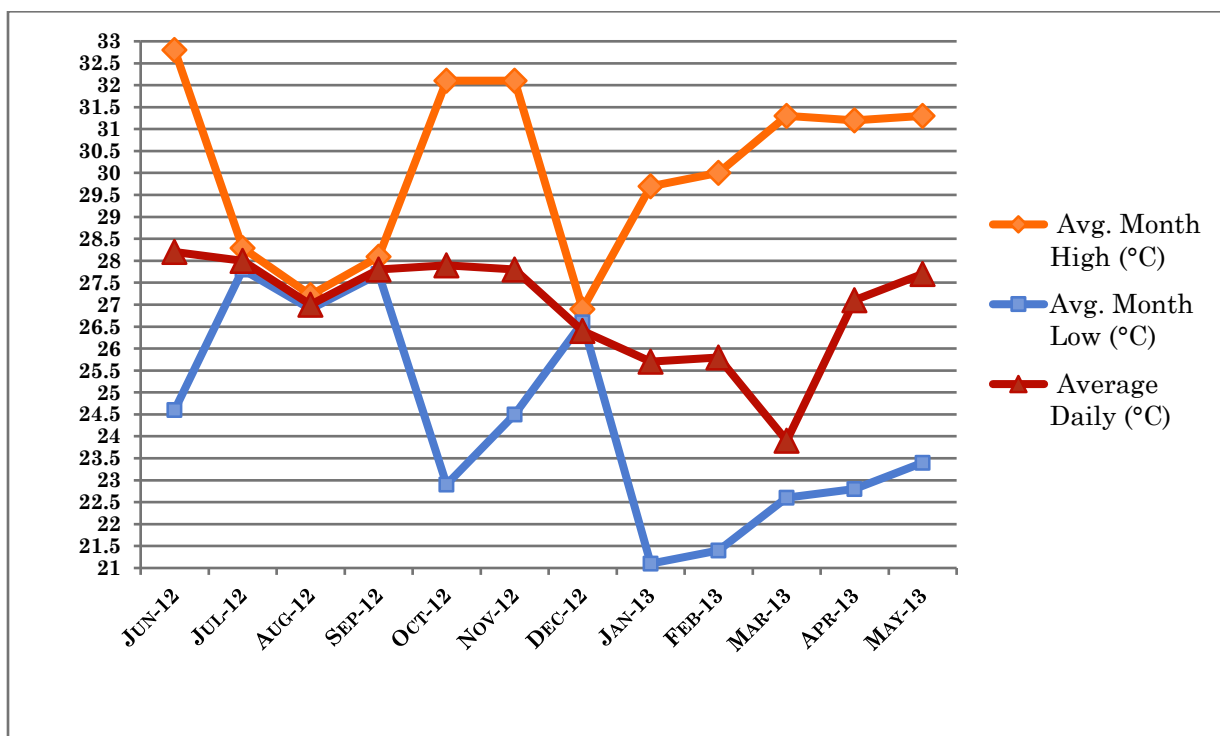
Graph 16: Monthly Highs, Lows and Average Temperatures recorded during the period June 2012 to May 2013.
