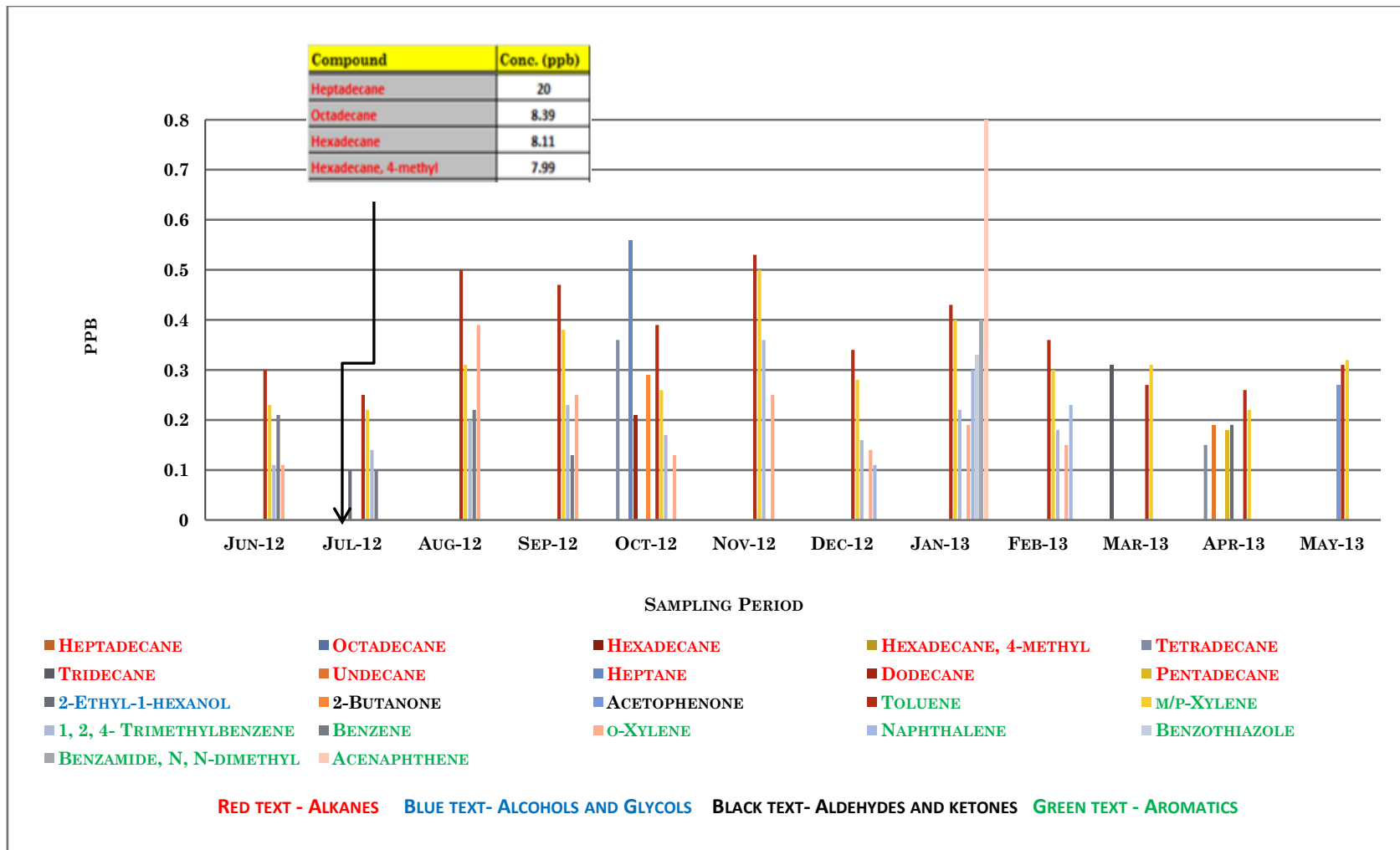
Graph 14: VOC compounds detected at Cypress Street during the study period June 2012 to May 2013. The compounds shown represent only those compounds covered in the laboratory accredited flexible scope and are not blank corrected.
