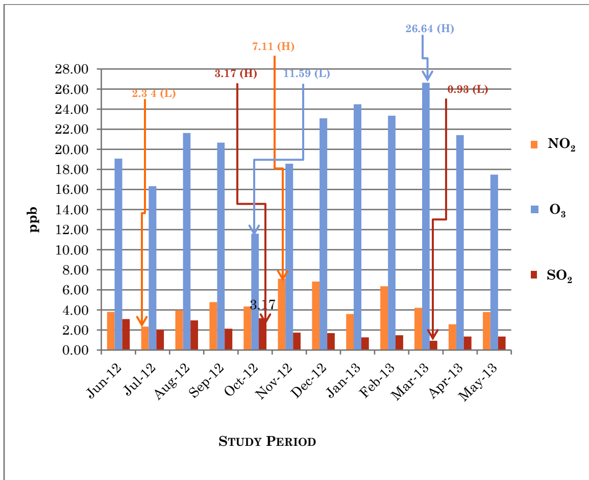
Graph 7: SO 2 , NO 2 and O 3 concentrations detected at Pickwick Gap, St. Michael. (H) represents the highest and (L) represents the lowest value detected.
